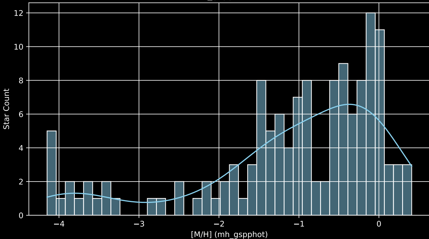
APOGEE DR17 Field: [162-60-C [M/H] (mh_gspphot) (n= 137)
