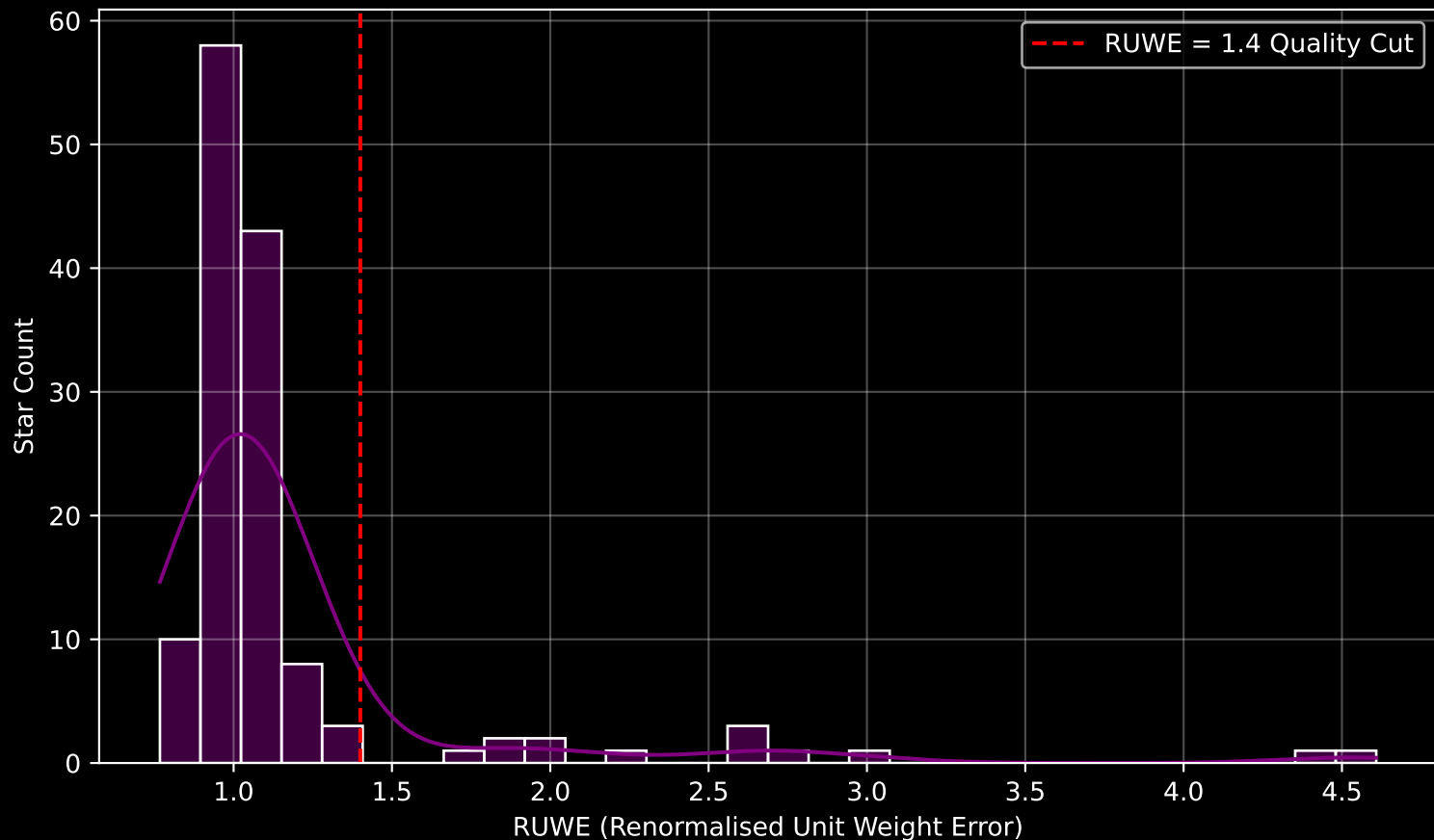
GAPOGEE DR17 Field [162-60-C] RUWE Distribution (n= 135)
