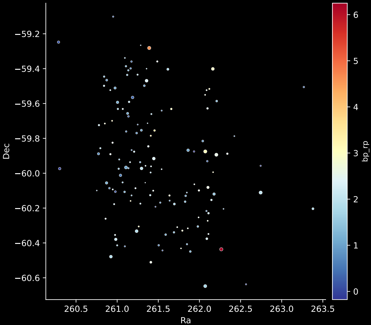
APOGEE DR17 Field: [162-60-C] Stars: 139
