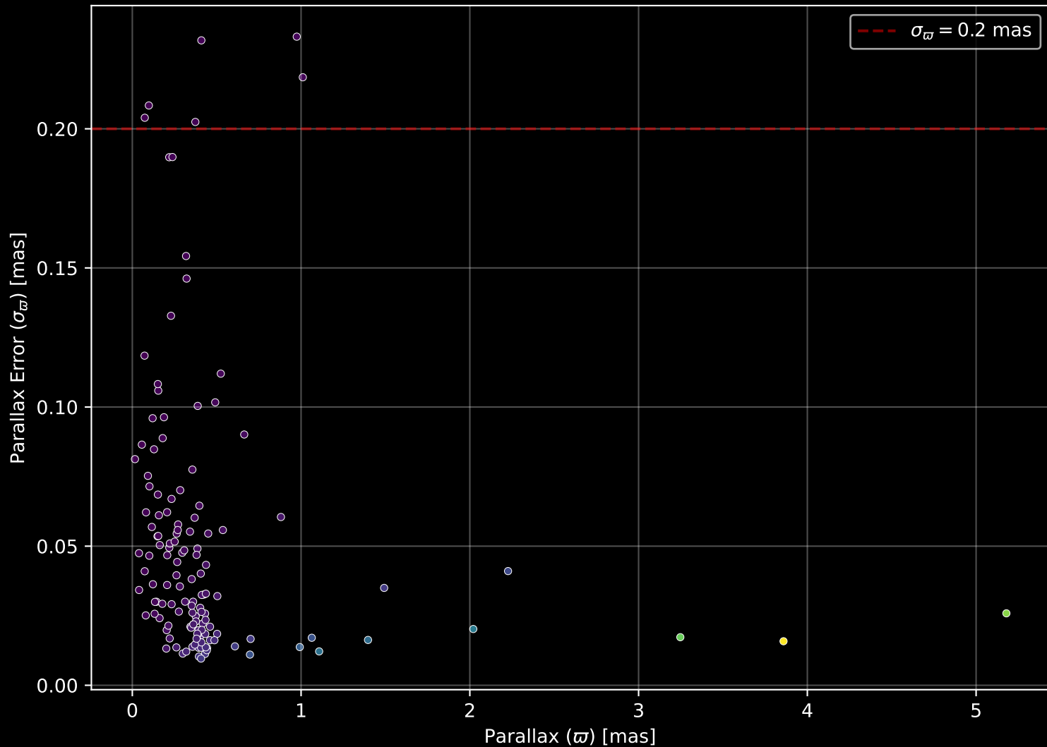
APOGEE DR17 Field: [162-60-C] Parallax Quality (n= 139)
