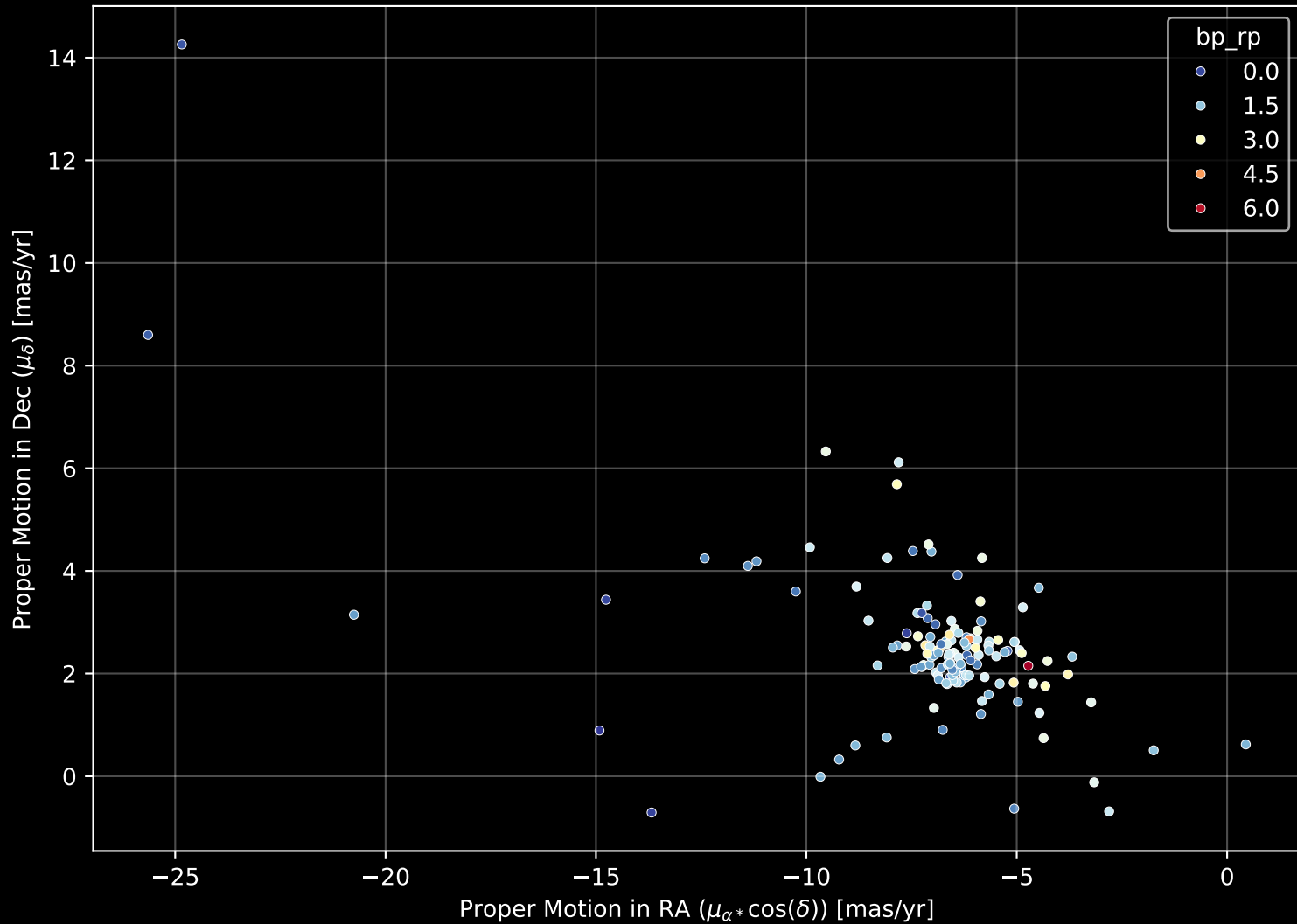
APOGEE DR17 Field: [162-60-C] Proper Motion Diagram (n= 139)
