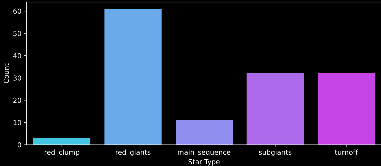
APOGEE DR17 Field: [162-60-C] Count plot of Star Type
