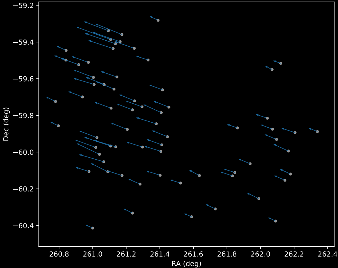
APOGEE DR17 Cluster 0 Proper Motion Vectors (n=67)
